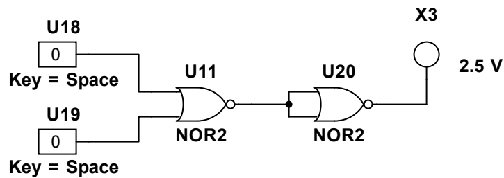
NOR AS OR
