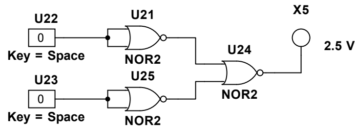
NOR AS AND
