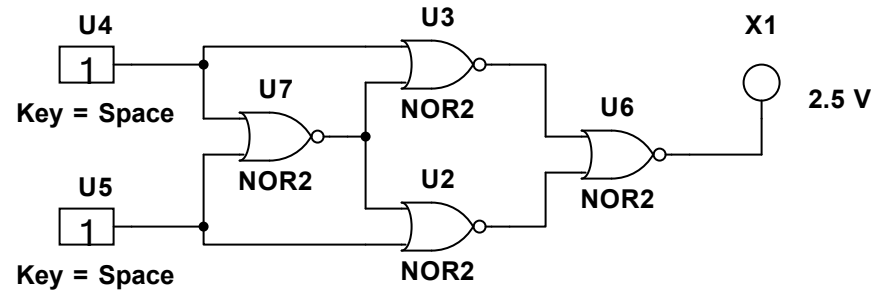
NOR AS XNOR
